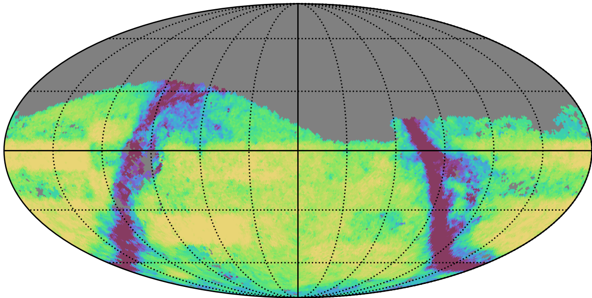
weather_cloudso16v3.4_10yrs Yr 3-4 g band: Exgal_CoaddM5
