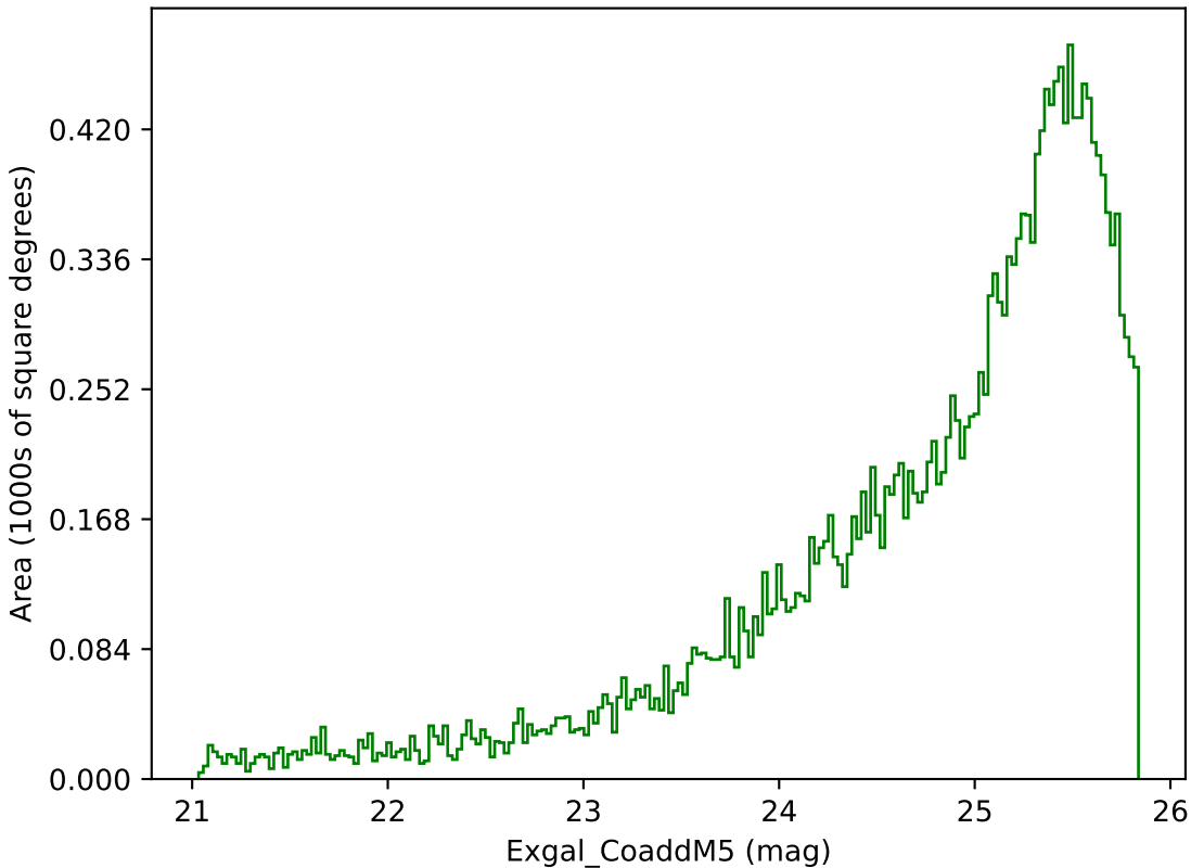
weather_cloudso16v3.4_10yrs Yr 3-4 g band: Exgal_CoaddM5
