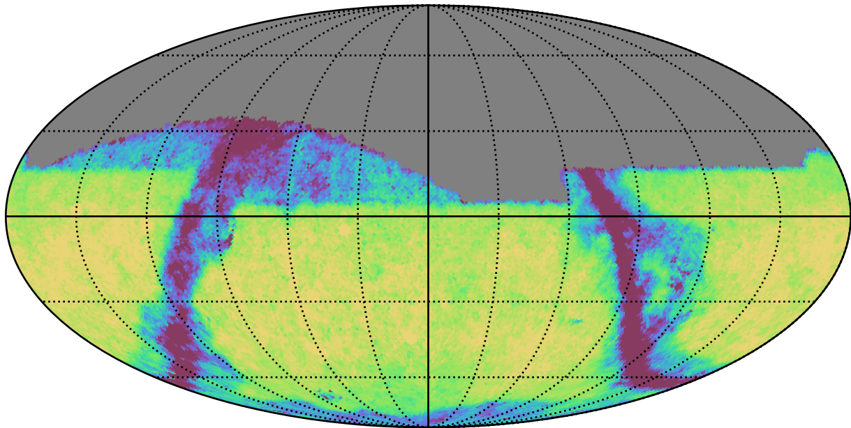
weather_cloudso16v3.4_10yrs Yr 1 z band: Exgal_CoaddM5
