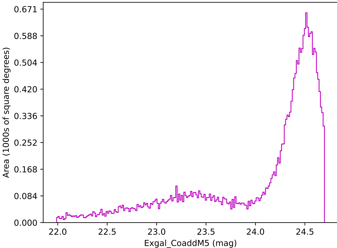
weather_cloudso16v3.4_10yrs Yr 1 z band: Exgal_CoaddM5
