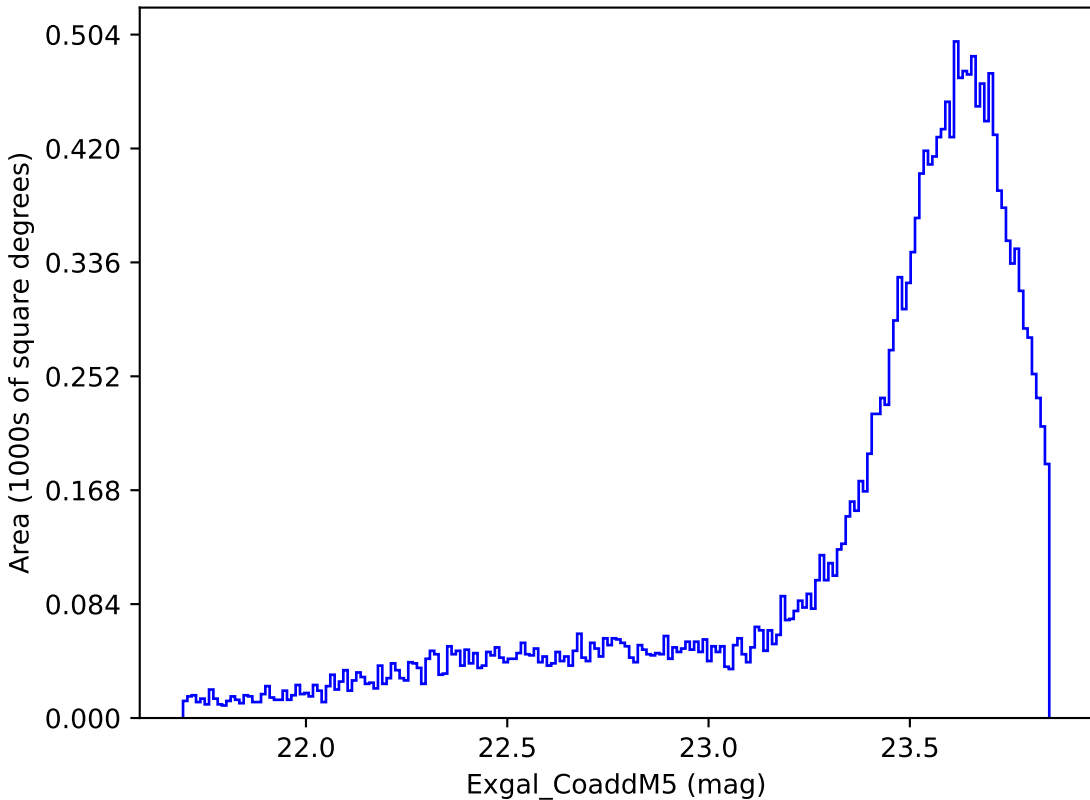
weather_cloudso16v3.4_10yrs Yr 1 y band: Exgal_CoaddM5
