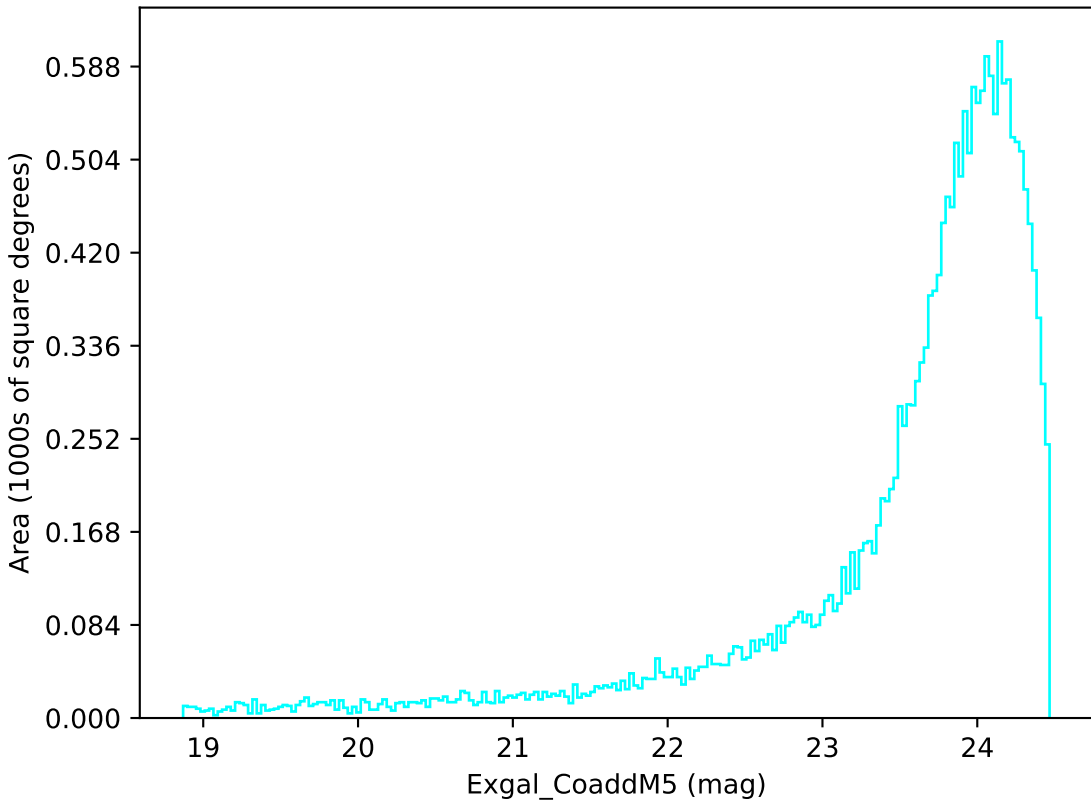
weather_cloudso16v3.4_10yrs Yr 1 u band: Exgal_CoaddM5
