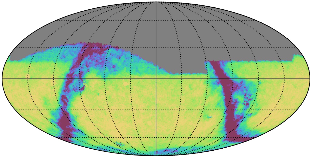
weather_cloudso16v3.4_10yrs Yr 1 r band: Exgal_CoaddM5
