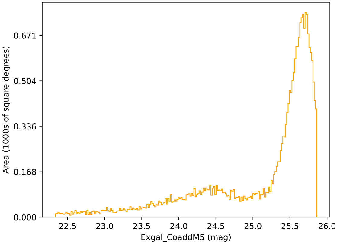
weather_cloudso16v3.4_10yrs Yr 1 r band: Exgal_CoaddM5
