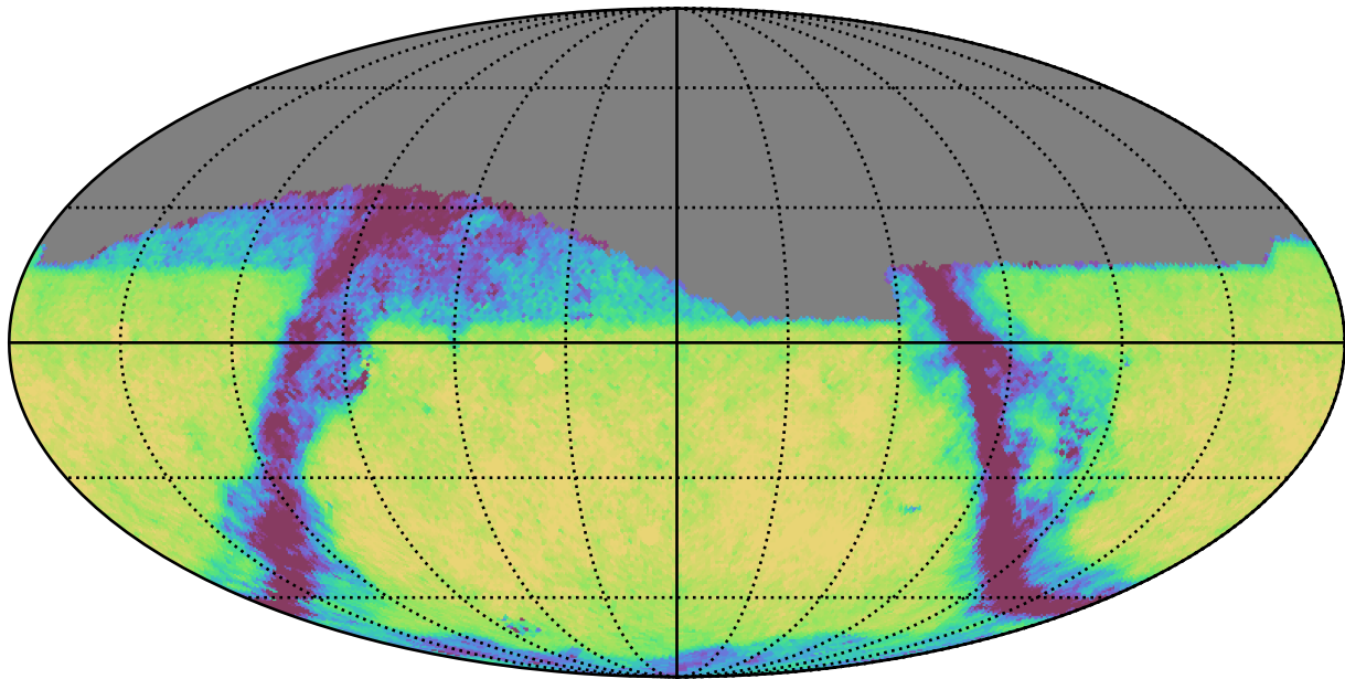
weather_cloudso16v3.4_10yrs Yr 1 i band: Exgal_CoaddM5
