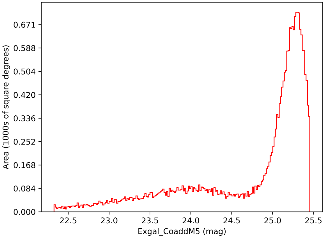
weather_cloudso16v3.4_10yrs Yr 1 i band: Exgal_CoaddM5
