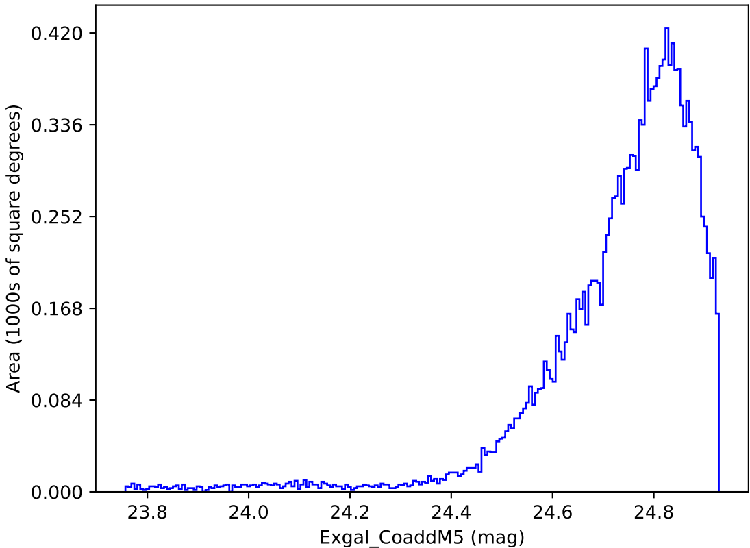
weather_cloudso16v3.4_10yrs WFD y band: Exgal_CoaddM5
