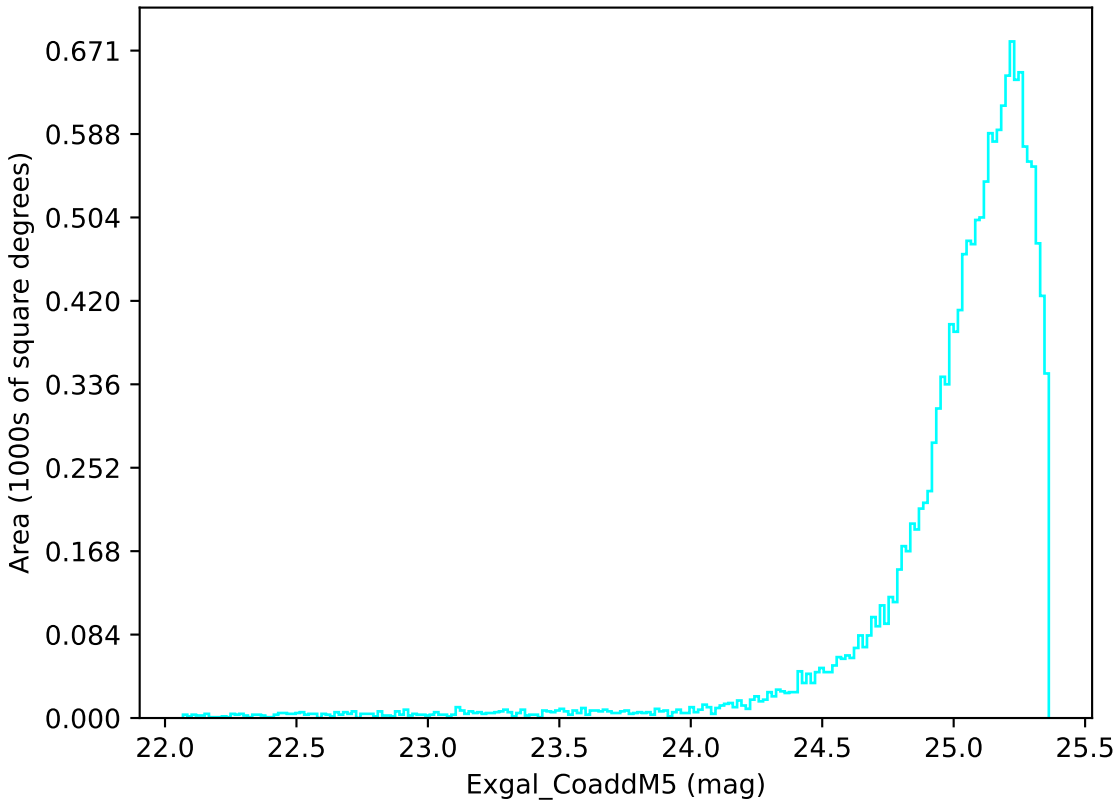
weather_cloudso16v3.4_10yrs WFD u band: Exgal_CoaddM5
