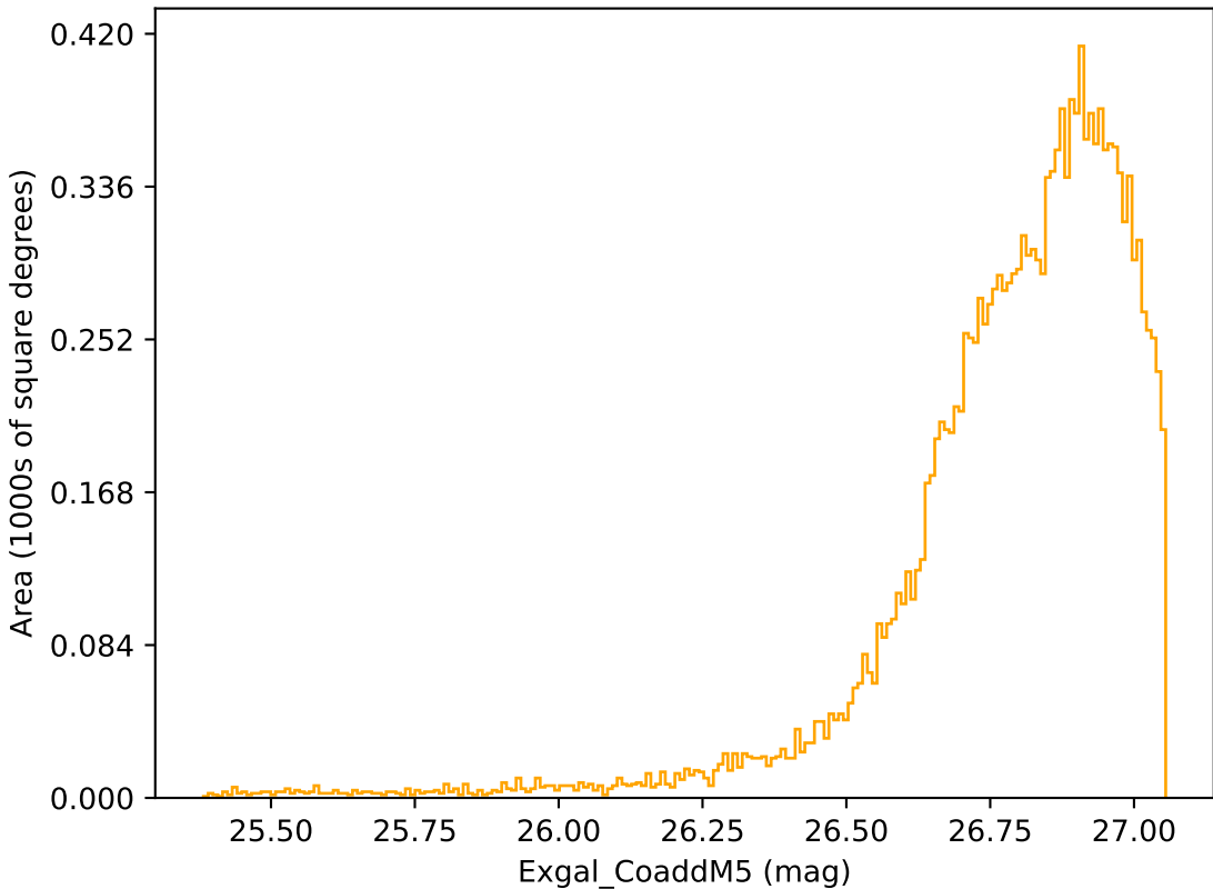
weather_cloudso16v3.4_10yrs WFD r band: Exgal_CoaddM5
