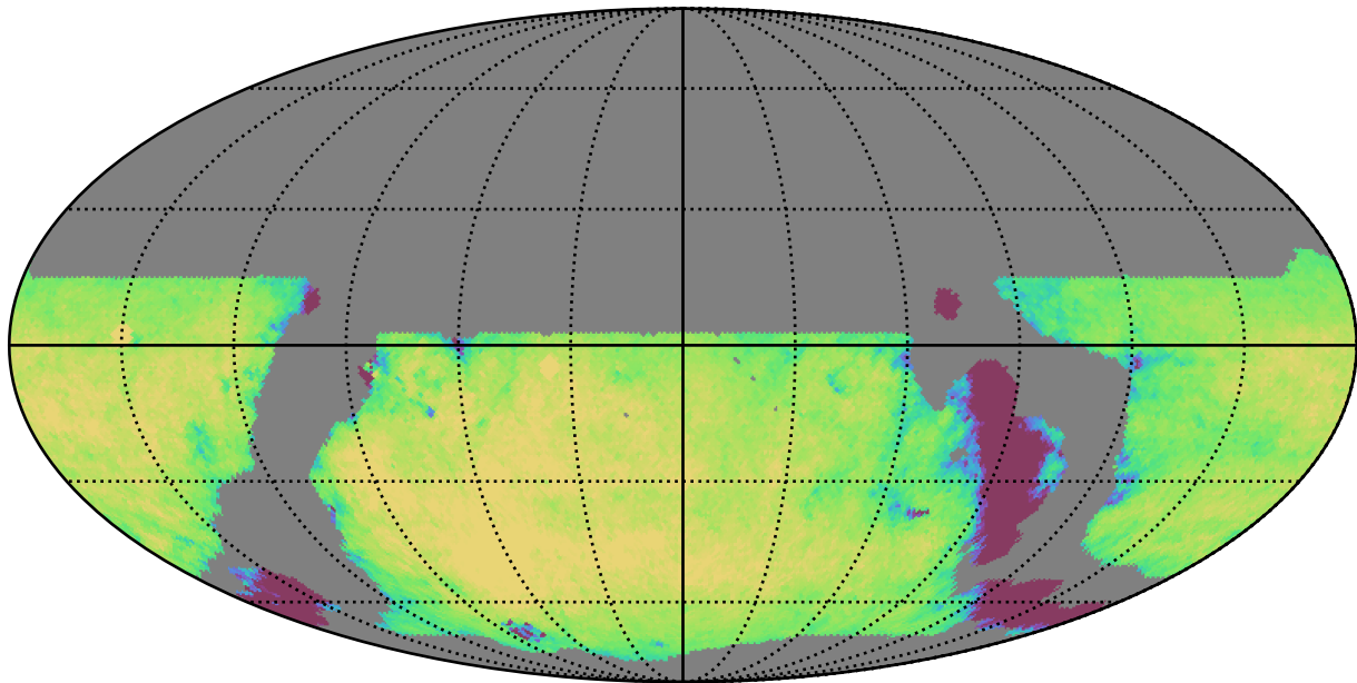
weather_cloudso16v3.4_10yrs WFD g band: Exgal_CoaddM5
