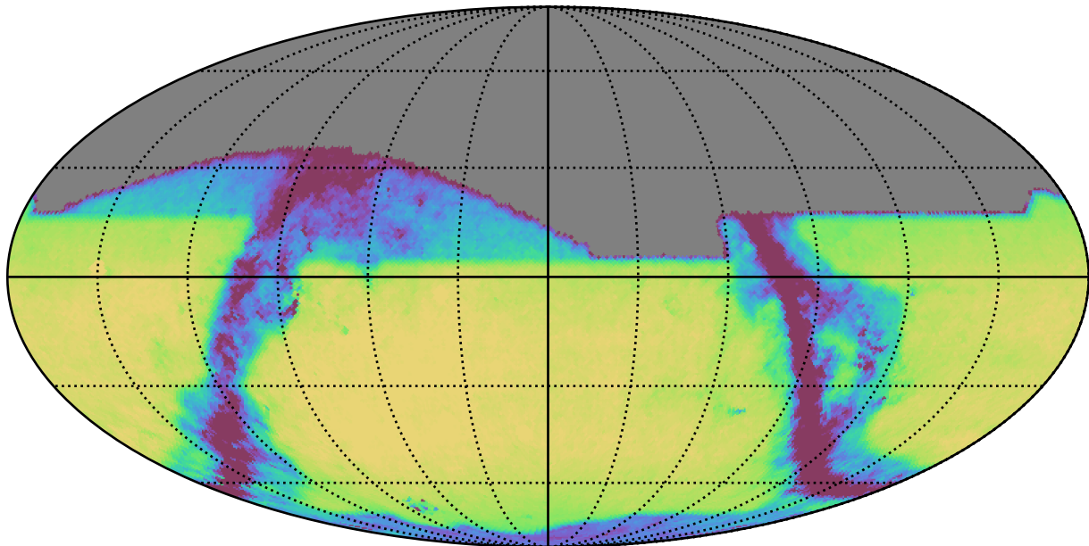
weather_cloudso16v3.4_10yrs All sky z band: Exgal_CoaddM5
