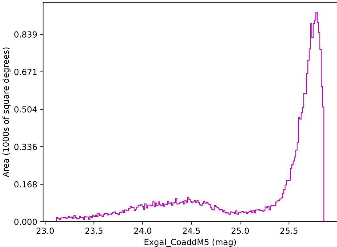
weather_cloudso16v3.4_10yrs All sky z band: Exgal_CoaddM5
