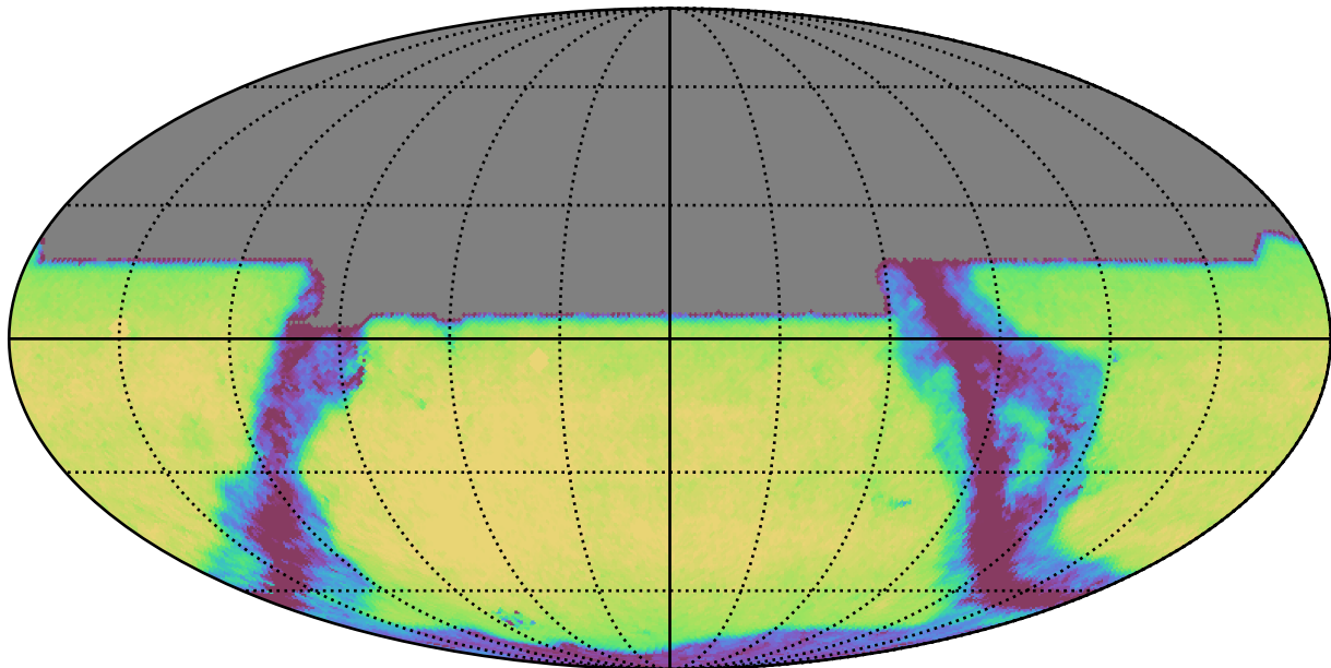
weather_cloudso16v3.4_10yrs All sky y band: Exgal_CoaddM5
