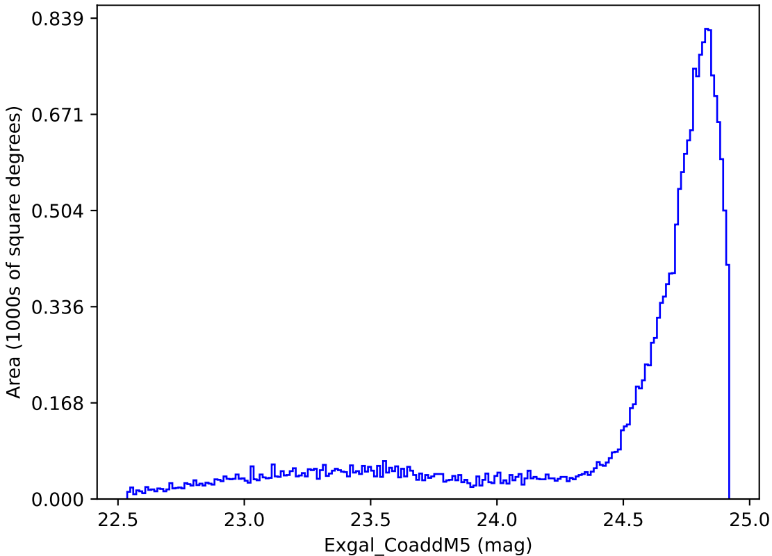
weather_cloudso16v3.4_10yrs All sky y band: Exgal_CoaddM5
