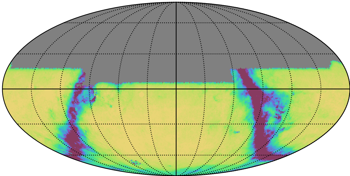
weather_cloudso16v3.4_10yrs All sky u band: Exgal_CoaddM5
