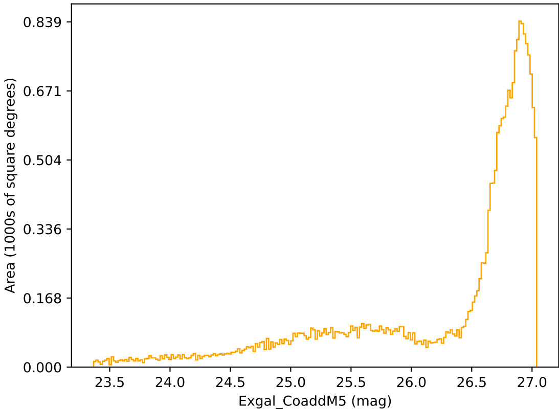
weather_cloudso16v3.4_10yrs All sky r band: Exgal_CoaddM5
