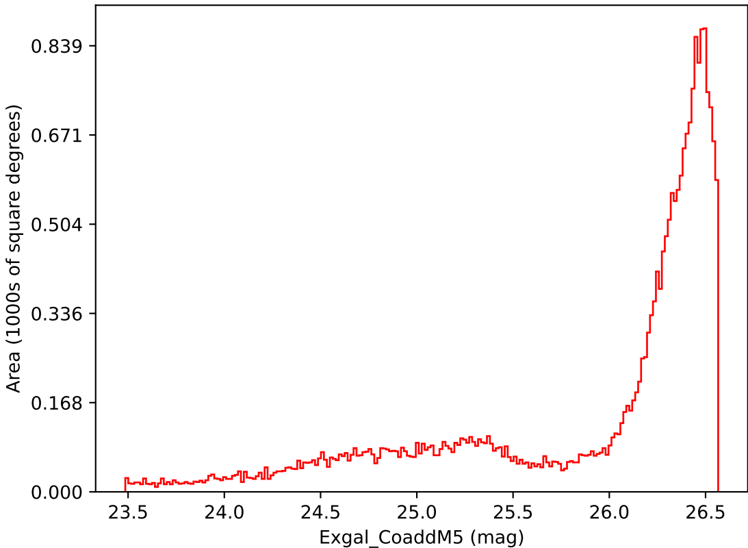
weather_cloudso16v3.4_10yrs All sky i band: Exgal_CoaddM5
