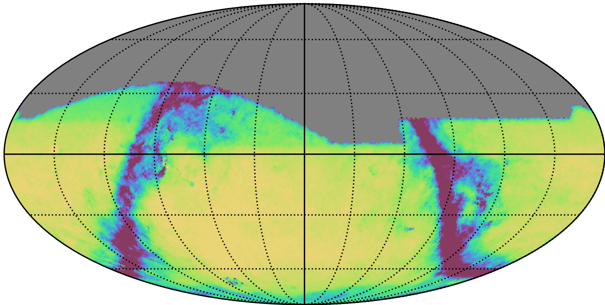
weather_cloudso16v3.4_10yrs All sky g band: Exgal_CoaddM5
