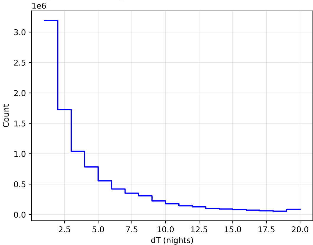
weather_cloudso16v3.4_10yrs All sky all bands: DeltaNight Histogram
