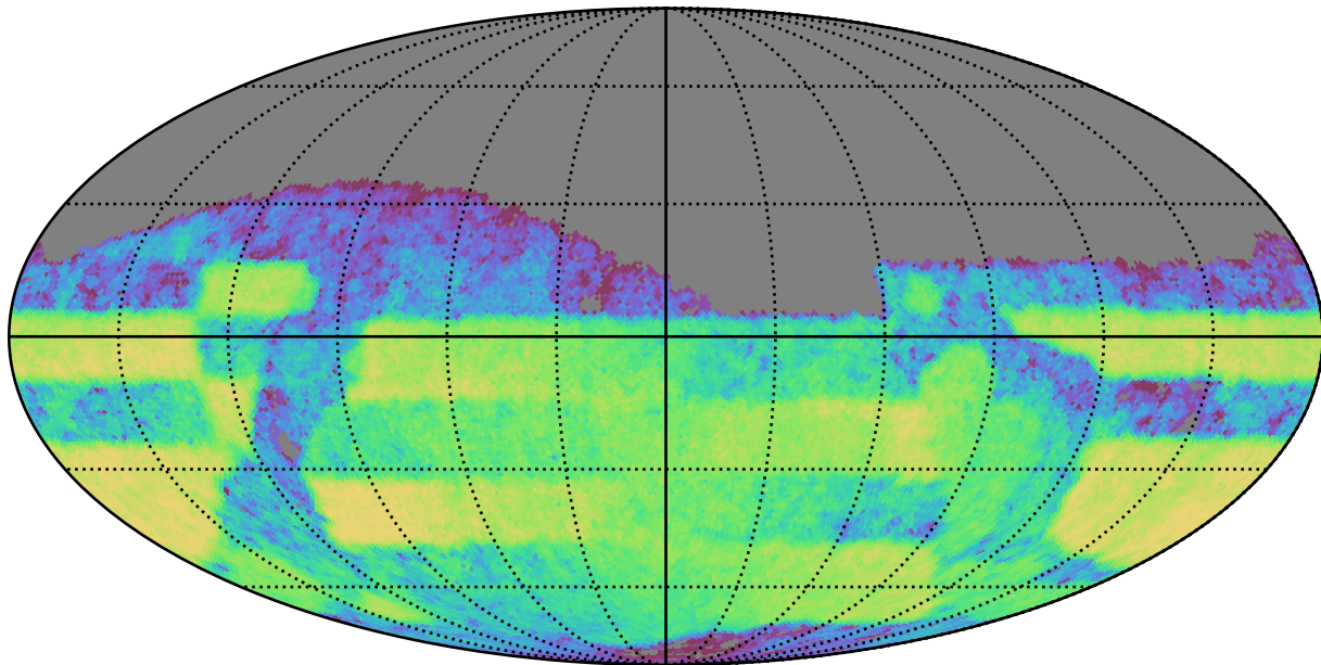
weather_cloudso16v3.4_10yrs Yr 3-4 z band: CoaddM5
