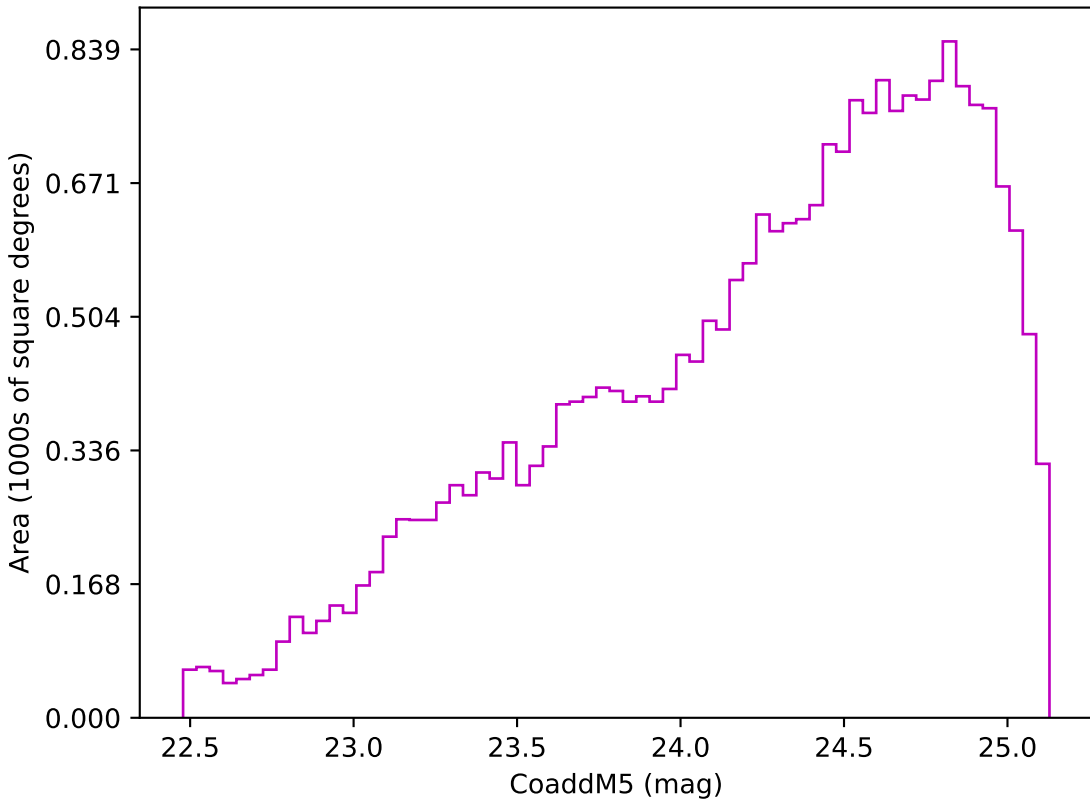
weather_cloudso16v3.4_10yrs Yr 3-4 z band: CoaddM5
