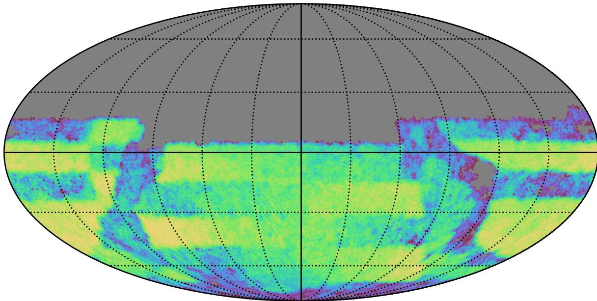
weather_cloudso16v3.4_10yrs Yr 3-4 y band: CoaddM5
