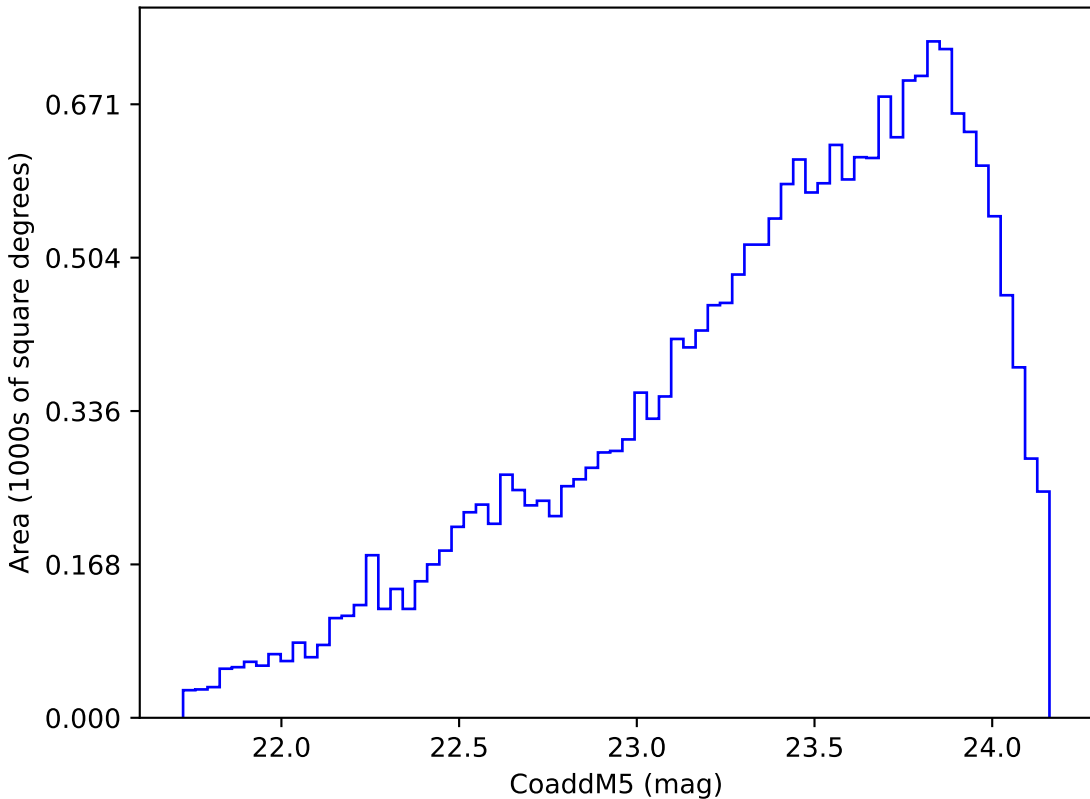
weather_cloudso16v3.4_10yrs Yr 3-4 y band: CoaddM5
