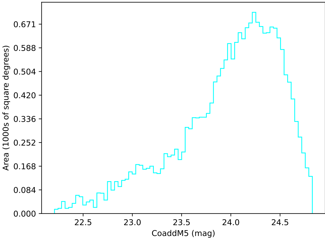
weather_cloudso16v3.4_10yrs Yr 3-4 u band: CoaddM5
