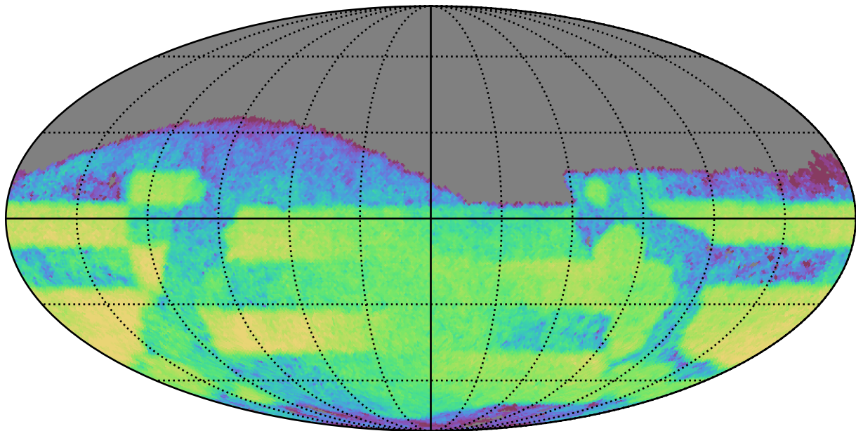
weather_cloudso16v3.4_10yrs Yr 3-4 r band: CoaddM5
