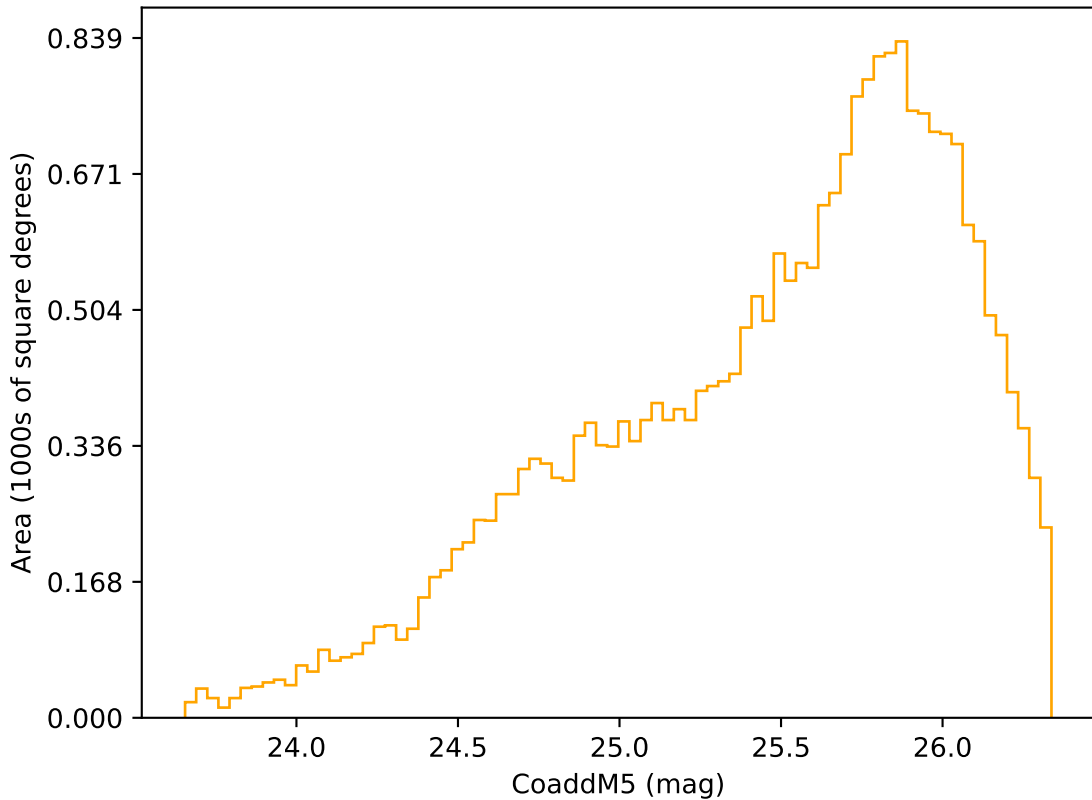
weather_cloudso16v3.4_10yrs Yr 3-4 r band: CoaddM5
