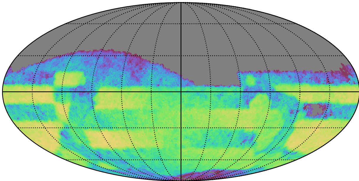
weather_cloudso16v3.4_10yrs Yr 3-4 i band: CoaddM5
