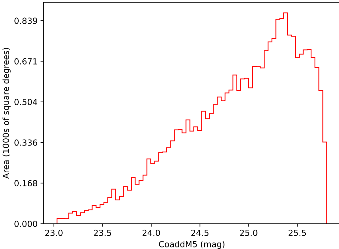
weather_cloudso16v3.4_10yrs Yr 3-4 i band: CoaddM5
