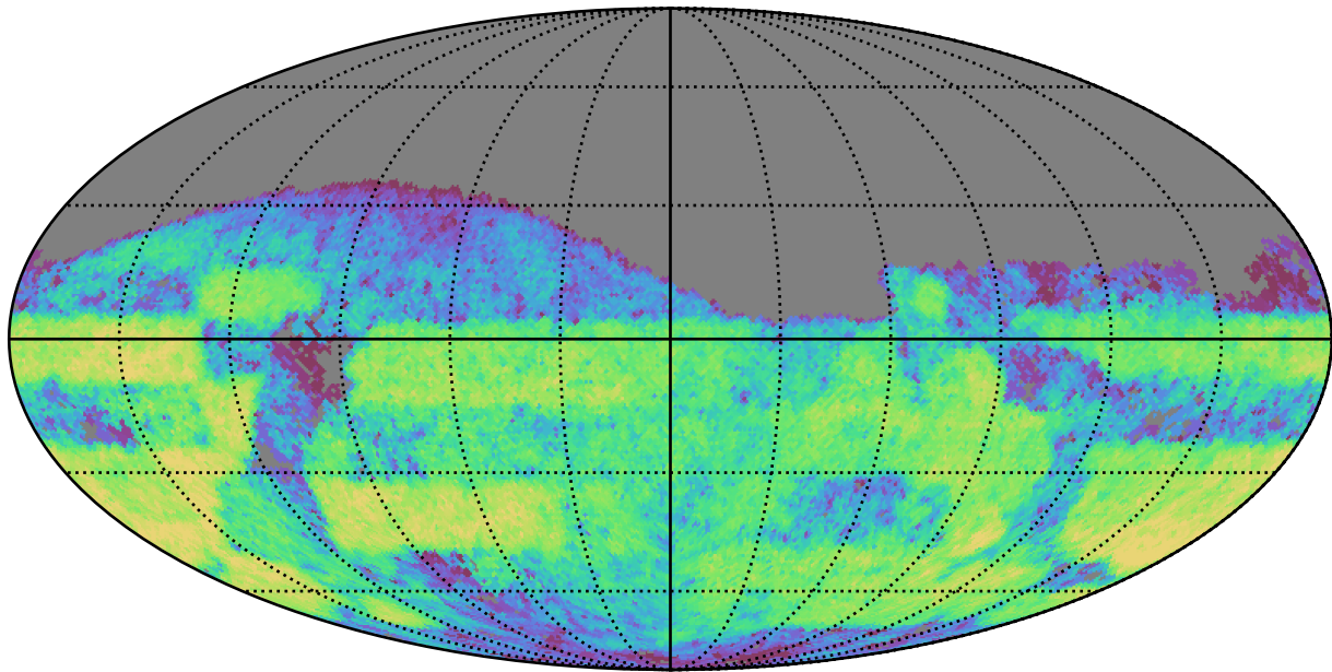
weather_cloudso16v3.4_10yrs Yr 3-4 g band: CoaddM5
