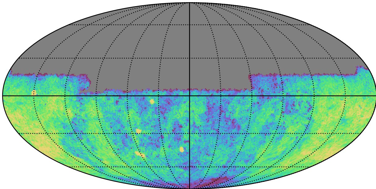
weather_cloudso16v3.4_10yrs Yr 1 u band: CoaddM5
