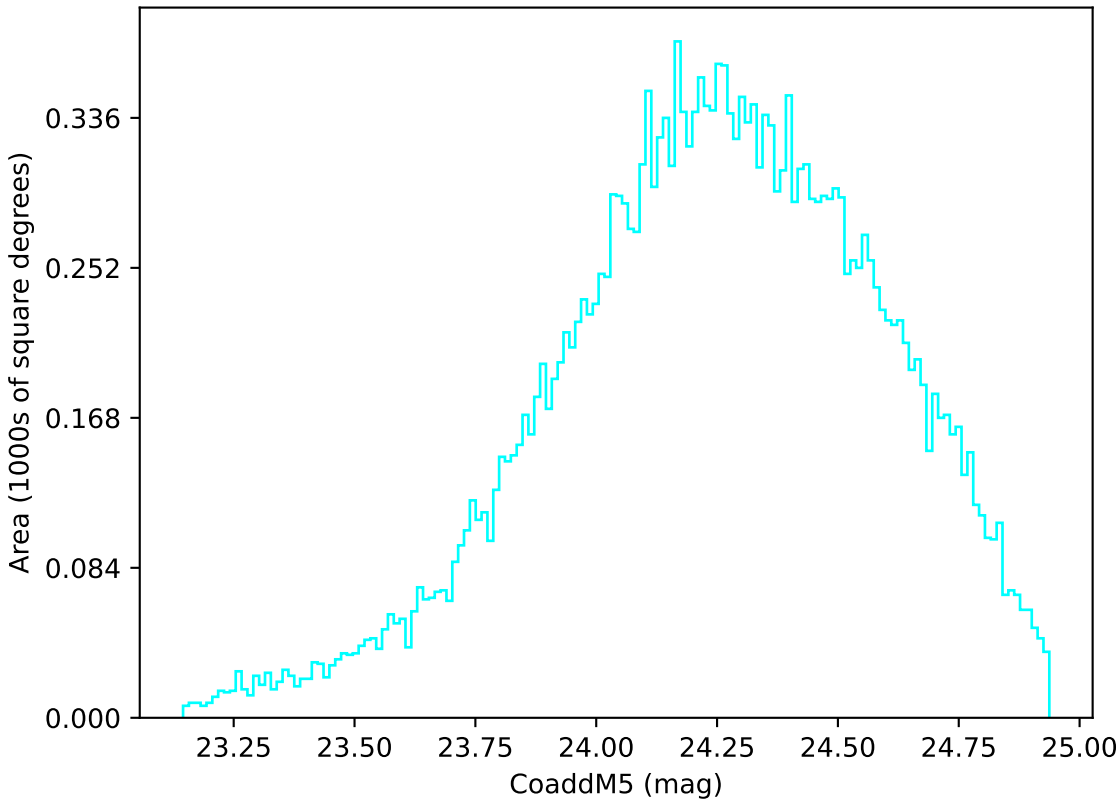
weather_cloudso16v3.4_10yrs Yr 1 u band: CoaddM5
