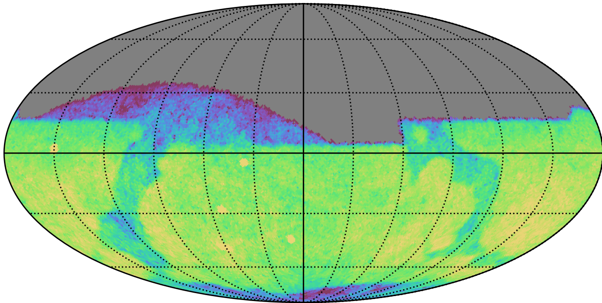
weather_cloudso16v3.4_10yrs Yr 1 r band: CoaddM5
