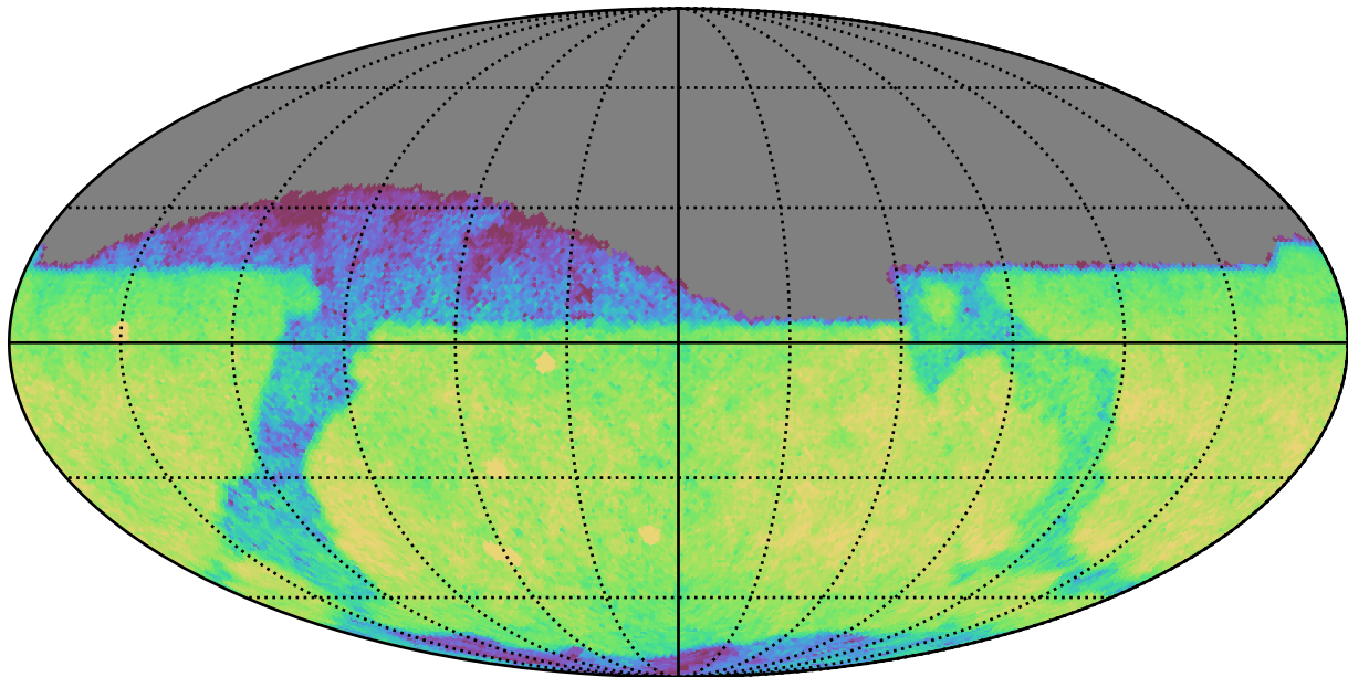
weather_cloudso16v3.4_10yrs Yr 1 i band: CoaddM5
