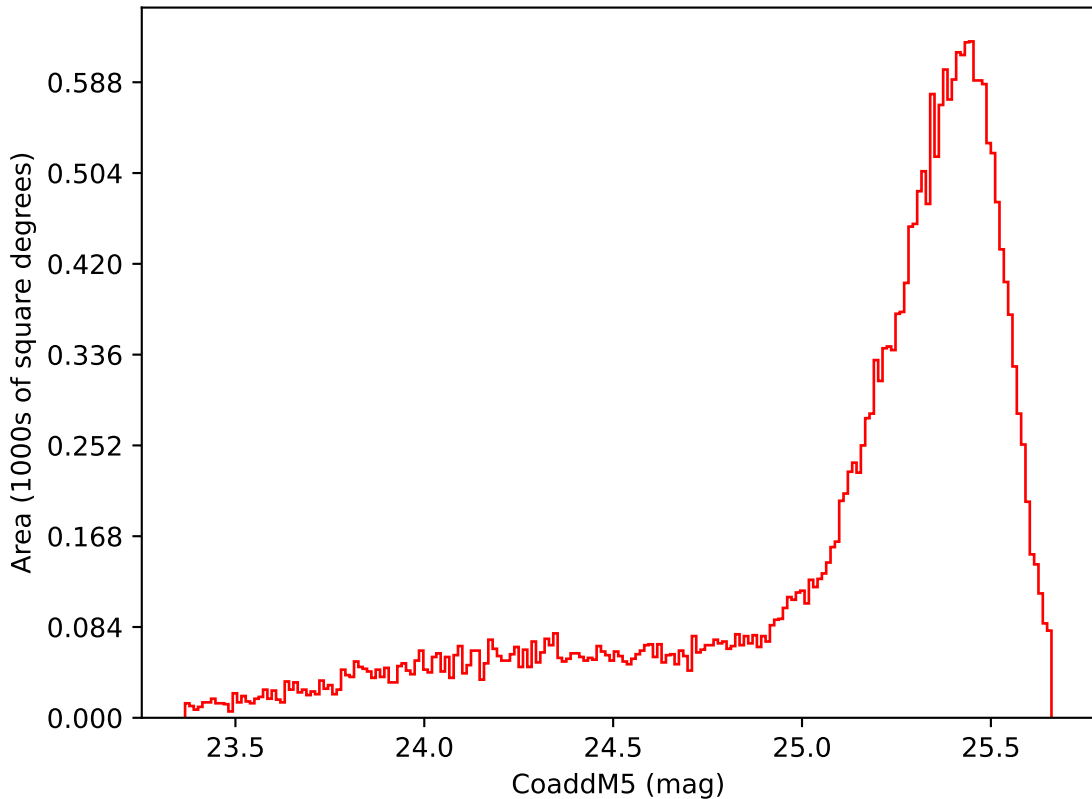
weather_cloudso16v3.4_10yrs Yr 1 i band: CoaddM5
