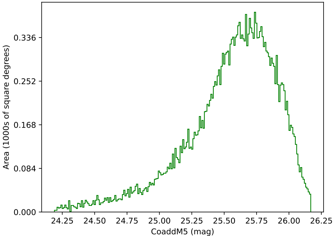
weather_cloudso16v3.4_10yrs Yr 1 g band: CoaddM5
