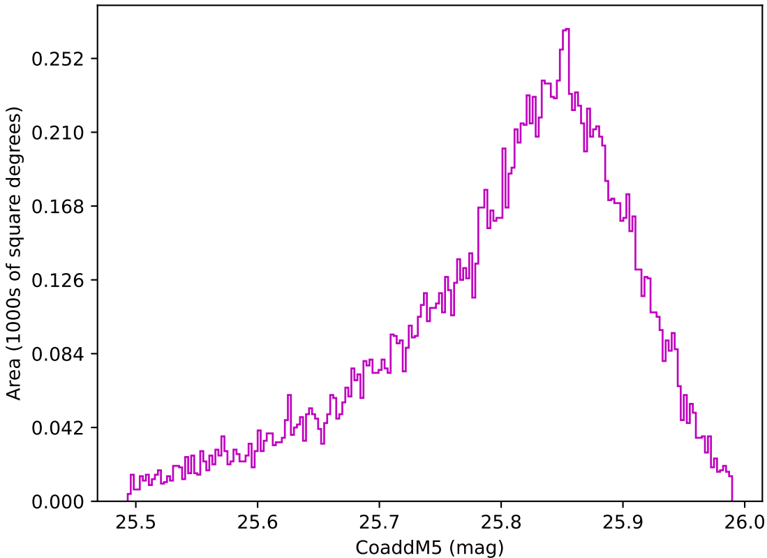
weather_cloudso16v3.4_10yrs WFD z band: CoaddM5
