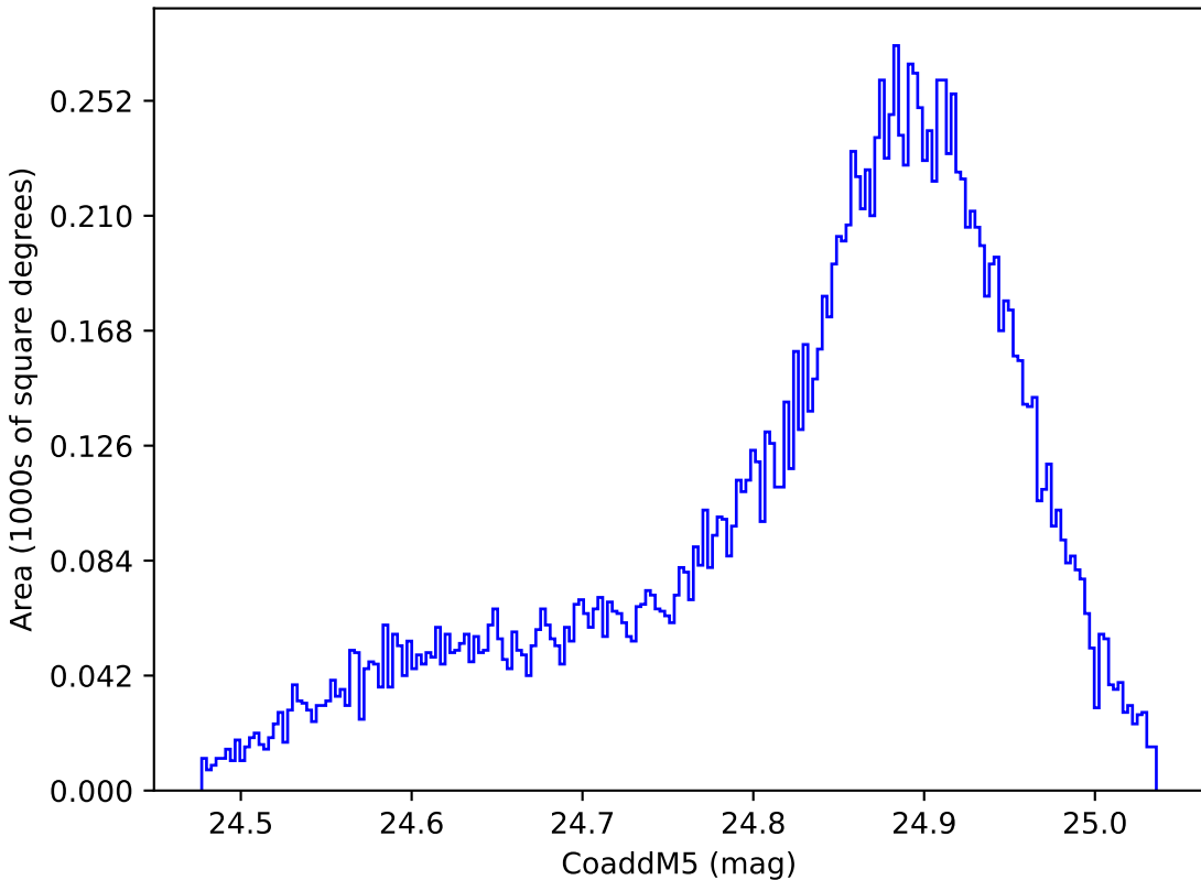
weather_cloudso16v3.4_10yrs WFD y band: CoaddM5
