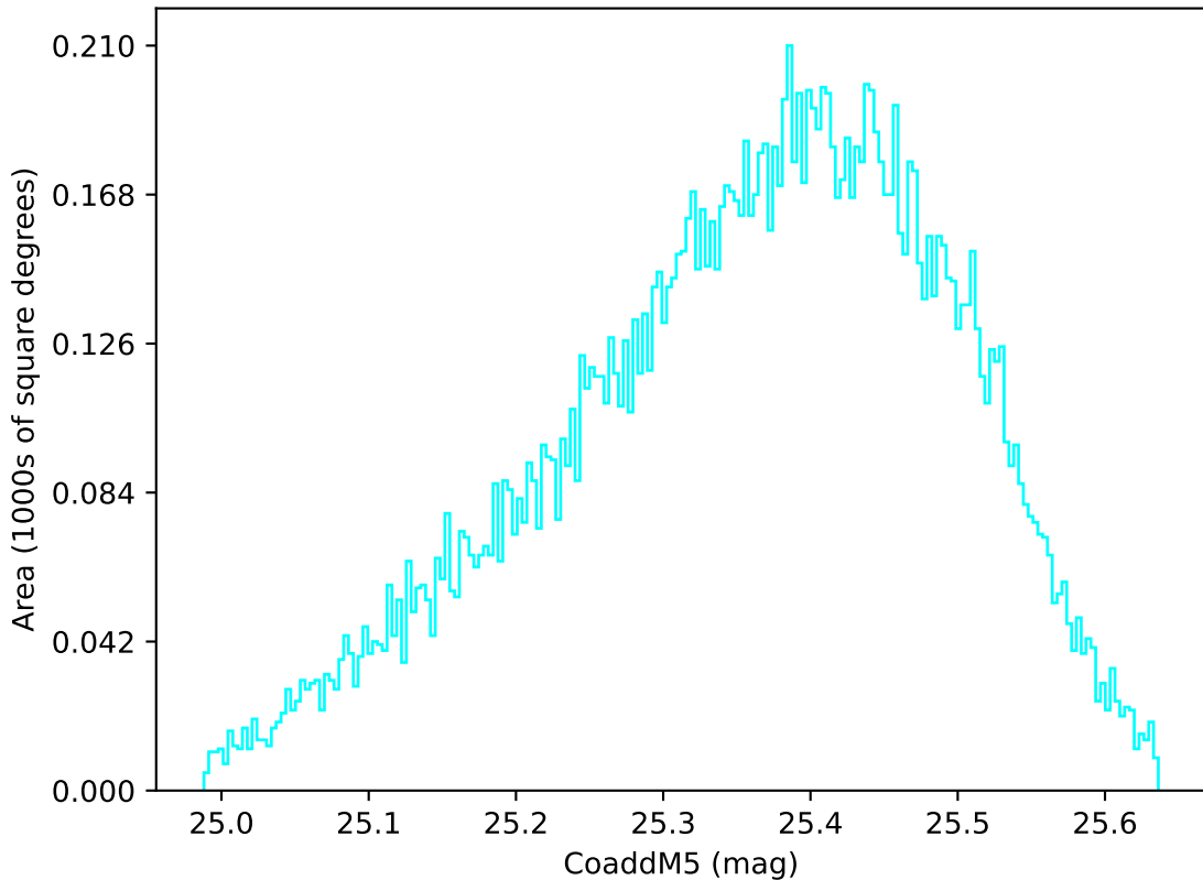
weather_cloudso16v3.4_10yrs WFD u band: CoaddM5
