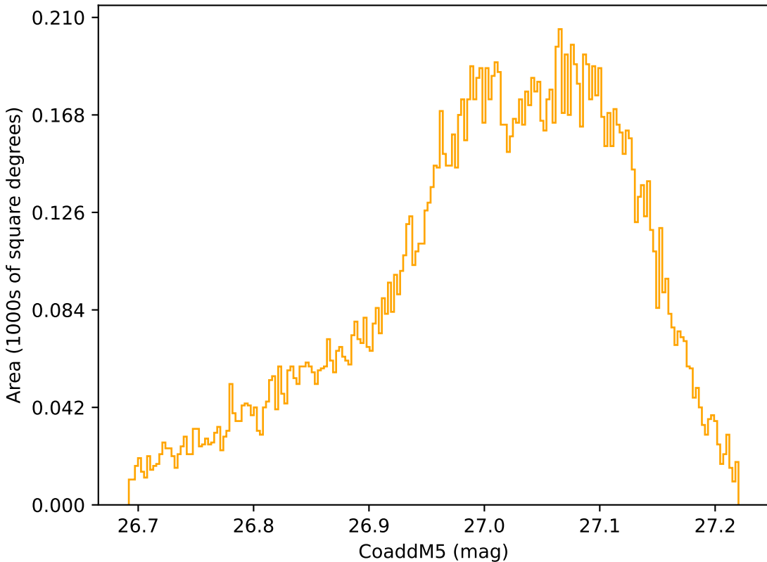
weather_cloudso16v3.4_10yrs WFD r band: CoaddM5
