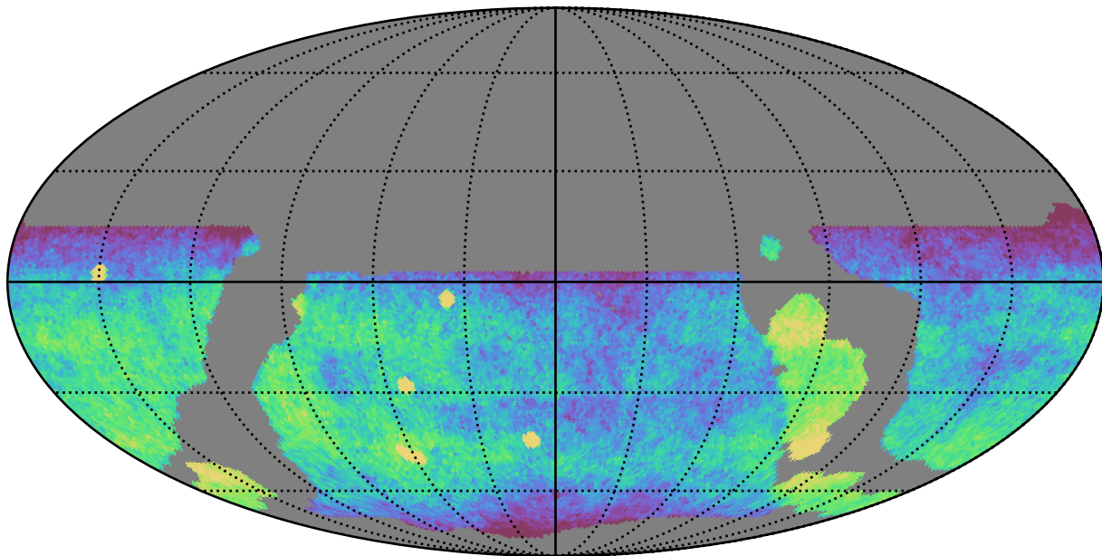
weather_cloudso16v3.4_10yrs WFD g band: CoaddM5
