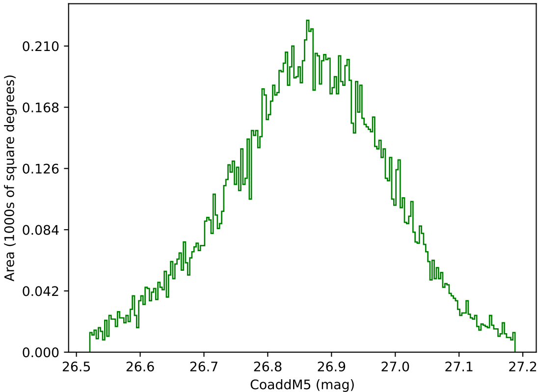
weather_cloudso16v3.4_10yrs WFD g band: CoaddM5
