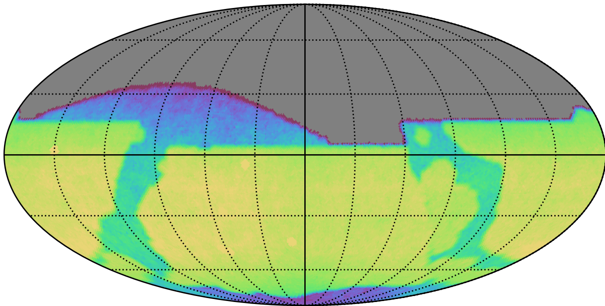
weather_cloudso16v3.4_10yrs All sky z band: CoaddM5
