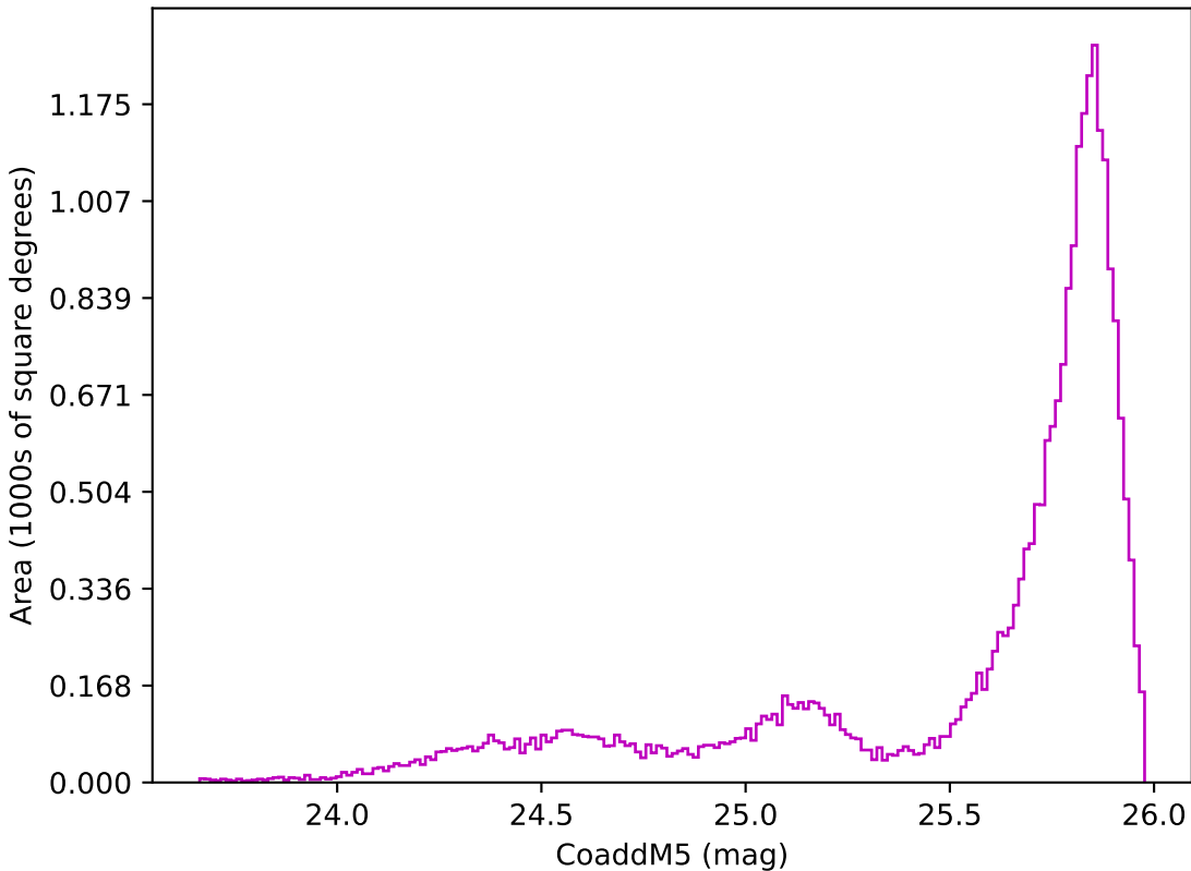
weather_cloudso16v3.4_10yrs All sky z band: CoaddM5
