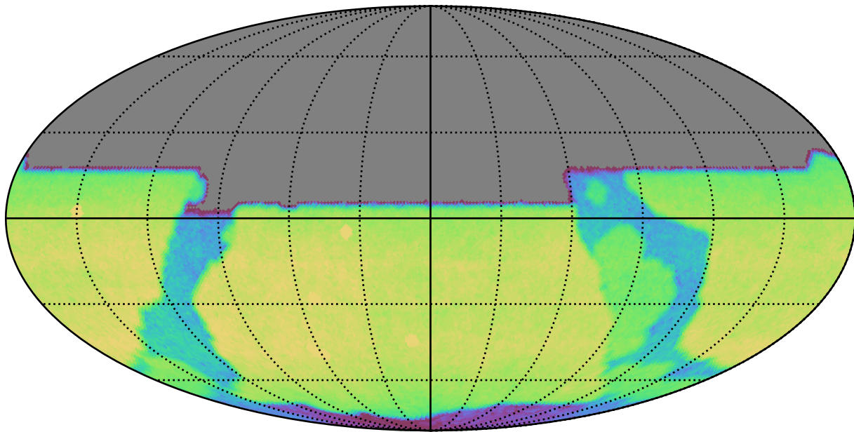
weather_cloudso16v3.4_10yrs All sky y band: CoaddM5
