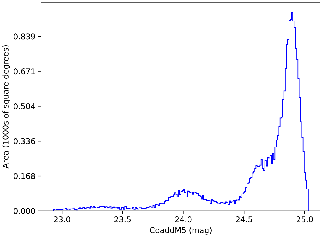
weather_cloudso16v3.4_10yrs All sky y band: CoaddM5
