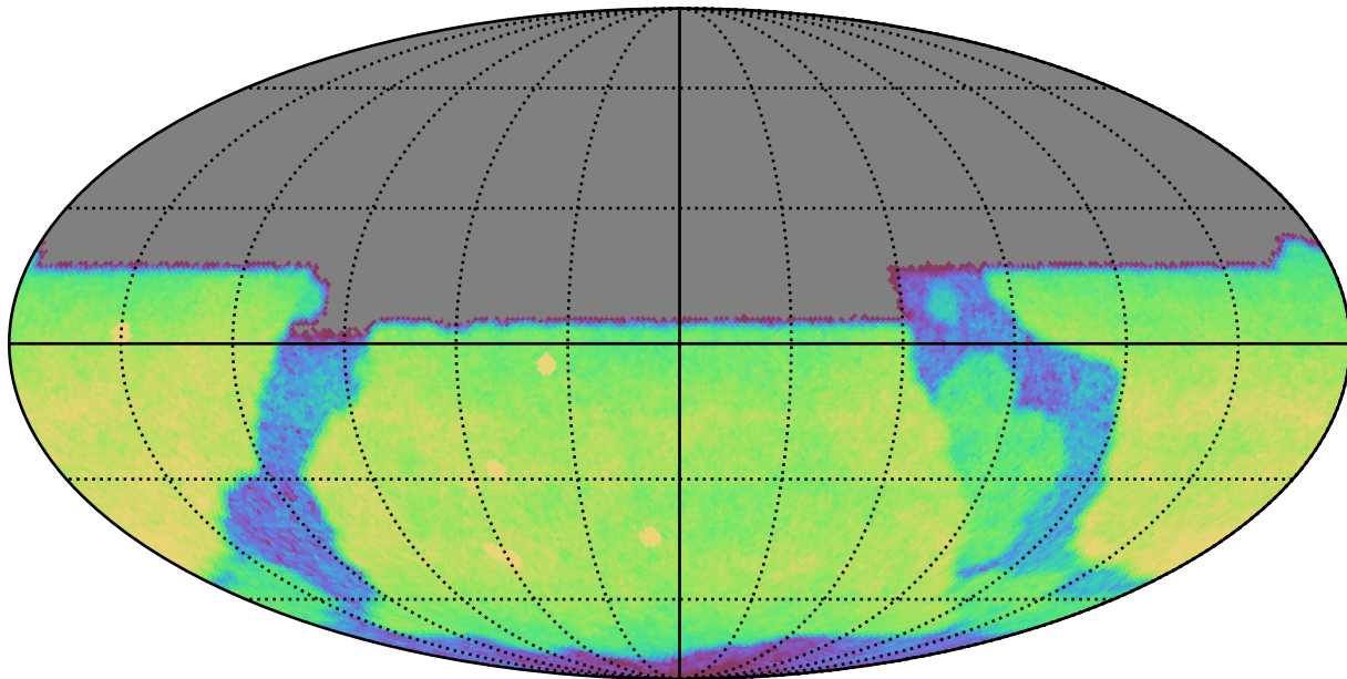
weather_cloudso16v3.4_10yrs All sky u band: CoaddM5
